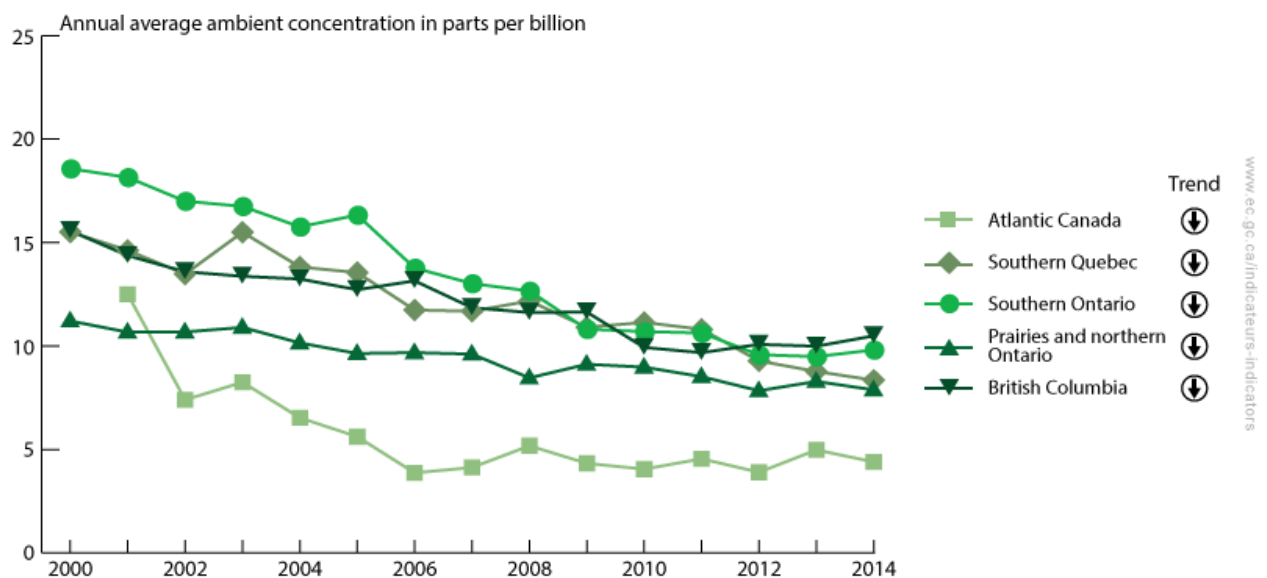
Figure 11. Regional nitrogen dioxide concentrations, 2000 to 2014
