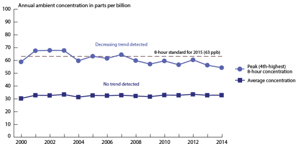
Figure 5. Ozone concentrations, Canada, 2000 to 2014
