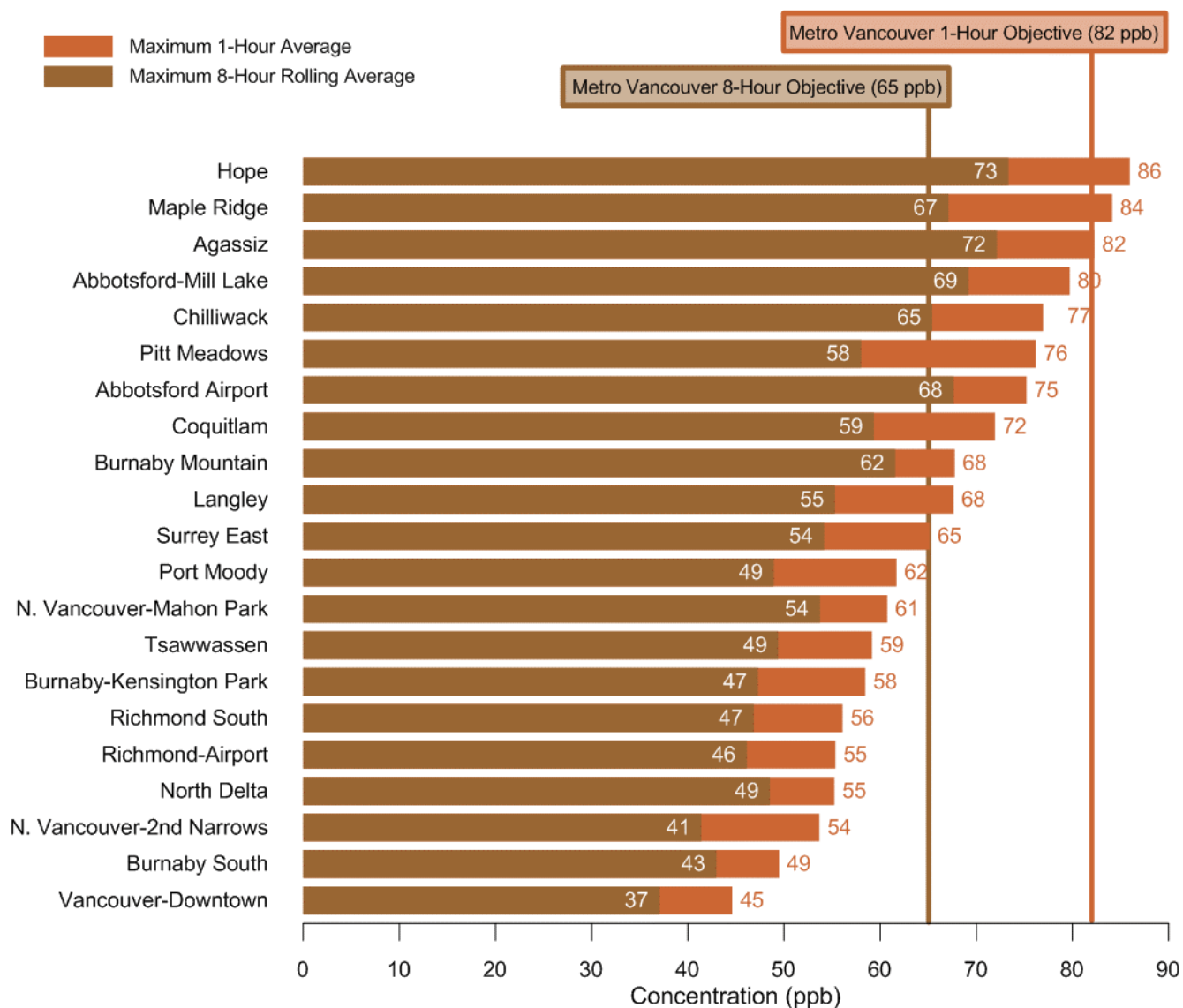
Figure 34: Ground-level ozone monitoring (1-hour and 8 hour), 2014.
