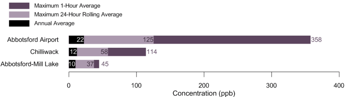
Figure 66: Ammonia monitoring, 2014.
