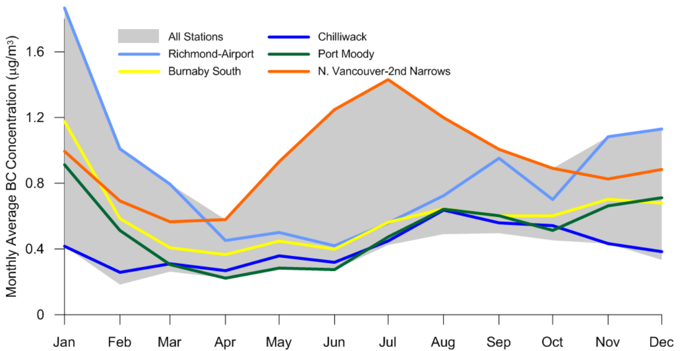
Figure 62: Monthly average black carbon, 2014.
