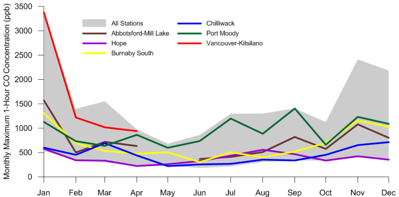
Figure 29: Monthly short-term peak carbon monoxide, 2014.
